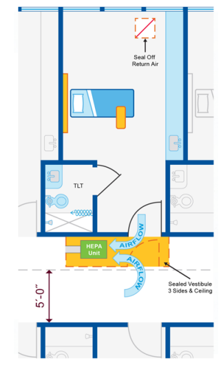
Figure 3. HEPA to corridor.
