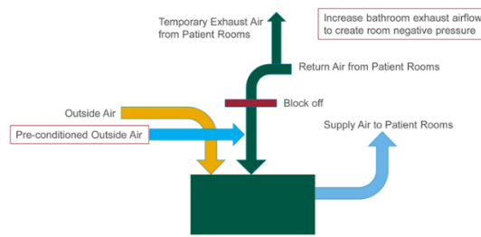
Figure 5. Example without Airside Economizer
